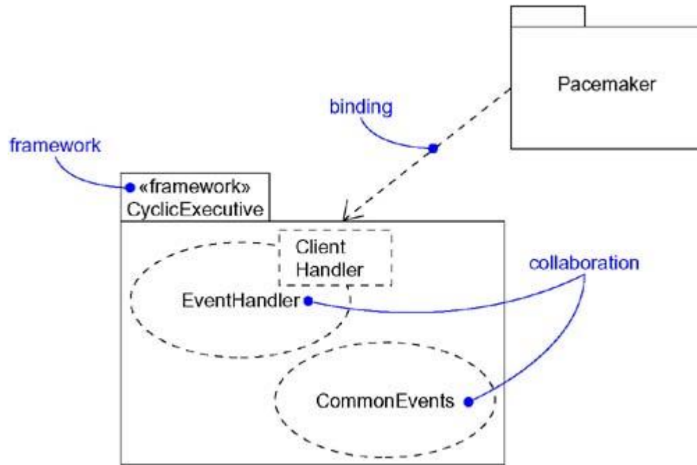
Figure 28-3 Frameworks
