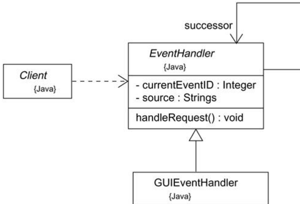
Figure 8-4 Forward Engineering
