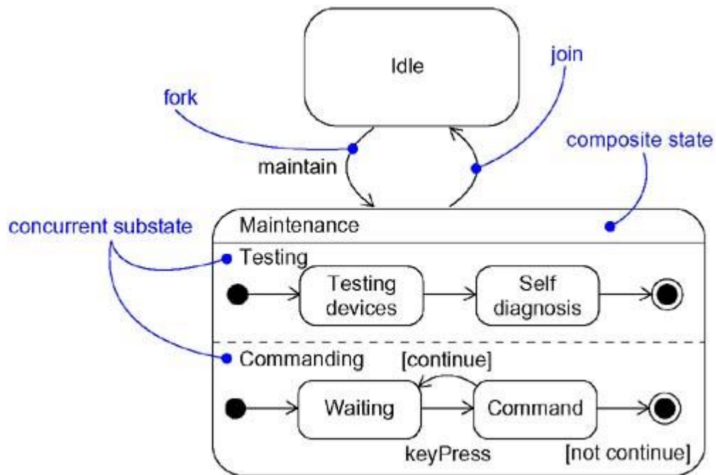
Figure 21-7 Concurrent Substates
