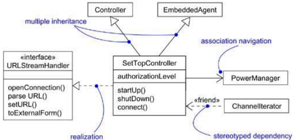
Figure 10-1 Advanced Relationships
