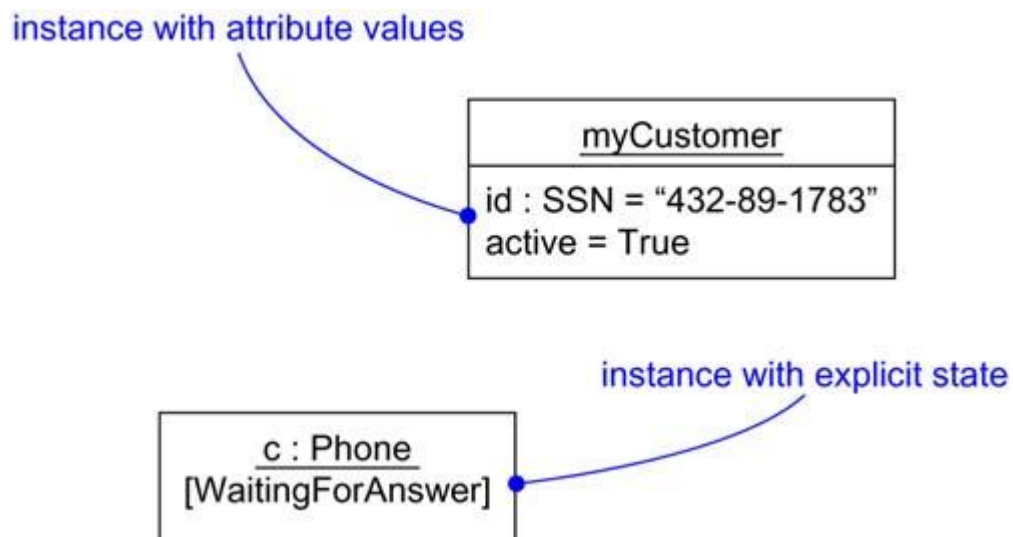
Figure 13-3 Object State
