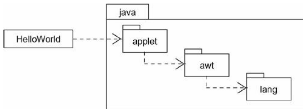
Figure 3-4 HelloWorld Packaging
