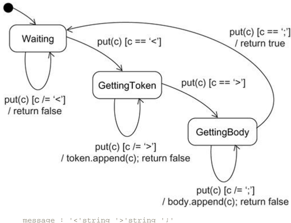
Figure 24-2 Modeling Reactive Objects
