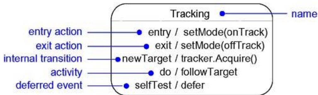
Figure 21-4 Advanced States and Transitions
