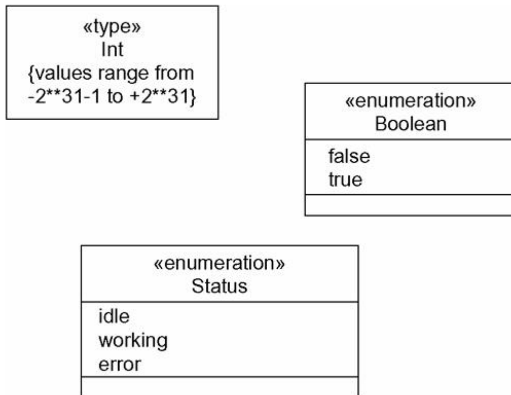
Figure 4-12 Modeling Primitive Types
